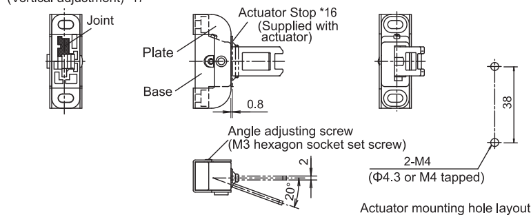
Actuator mounting hole layout
