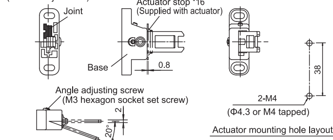
Actuator mounting hole layout
