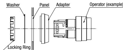
Washer
