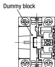
3 contact blocks
