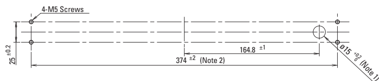
Mounting Hole Layout
