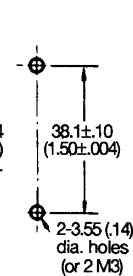
Mounting holes
