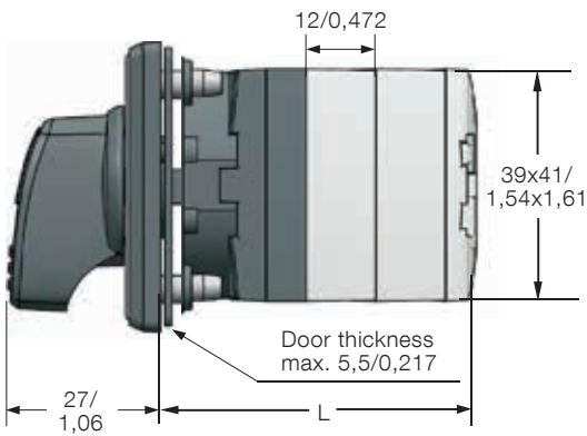
Screw mounting type, IP66
