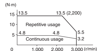
R88M-G1K020T (1 kW)
