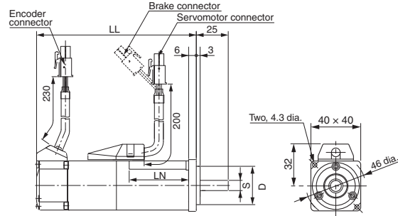
Servo motor with standard connector
