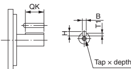
(Dimensions of shaft end with key and tap)
