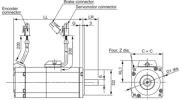
Servo motor with circular connector
