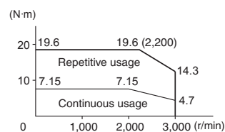
R88M-G1K520T (1.5 kW)
