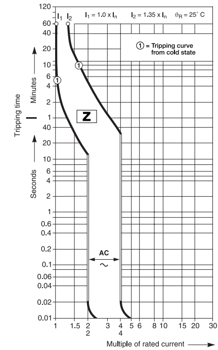
Z characteristic
