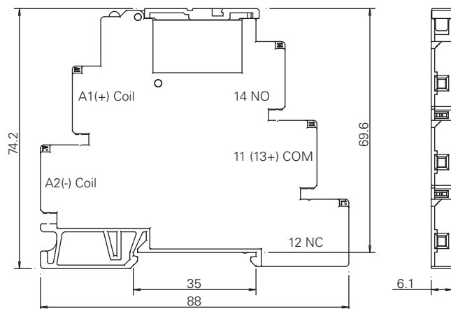
RV8H-S Spring Clamp Terminals
