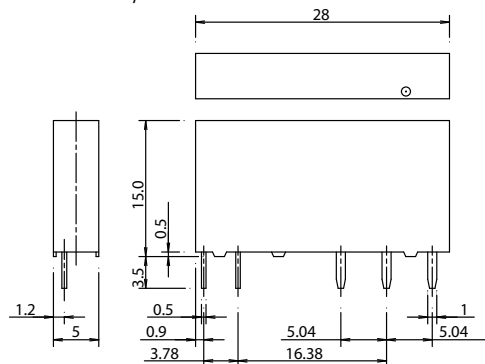
RV1H-G Relay
