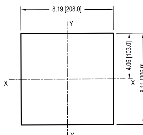
T7 3 & 4 POLE CUTOUT FOR DOOR COMPARTMENT
