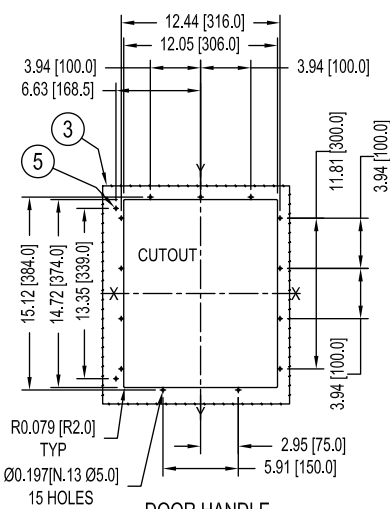
DOOR HANDLE DRILLING
