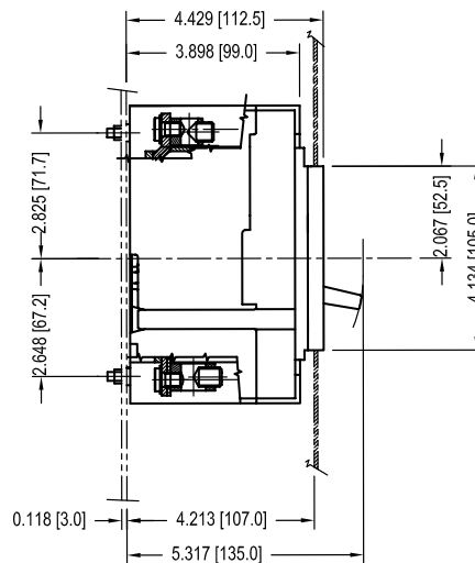
T3S 3 & 4 POLE SIDE VIEW WITHOUT FLANGE
