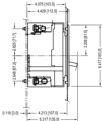
T3S 3 & 4 POLE SIDE VIEW WITH FLANGE
