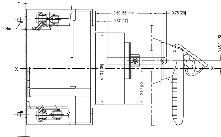
SIDE VIEW
