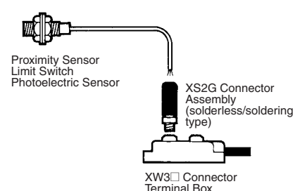
Pre-wired Type
