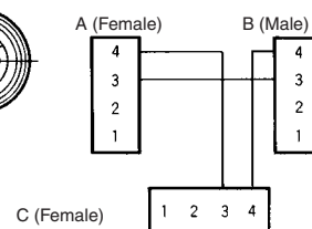
Internal Connections
