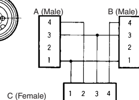
Internal Connections
