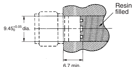
Mounted Dimensions
