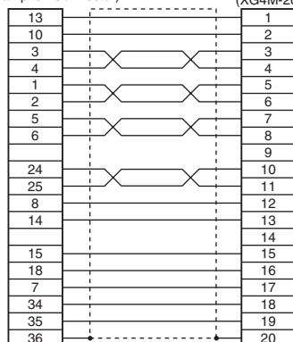
XW2Z-100J-B4
