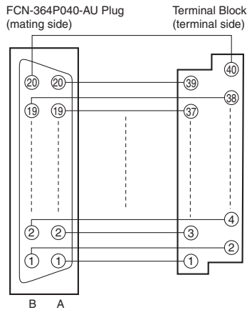
Wiring Diagram
