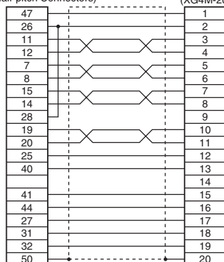
XW2Z-100J-B5
