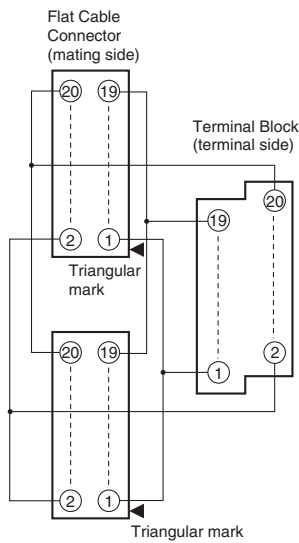
Wiring Diagram
