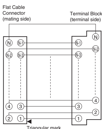
Wiring Diagram
