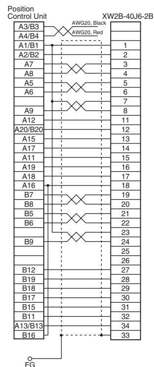
XW2Z-100J-A21 (for the R7D-AP and R88D-UEP□□□)
