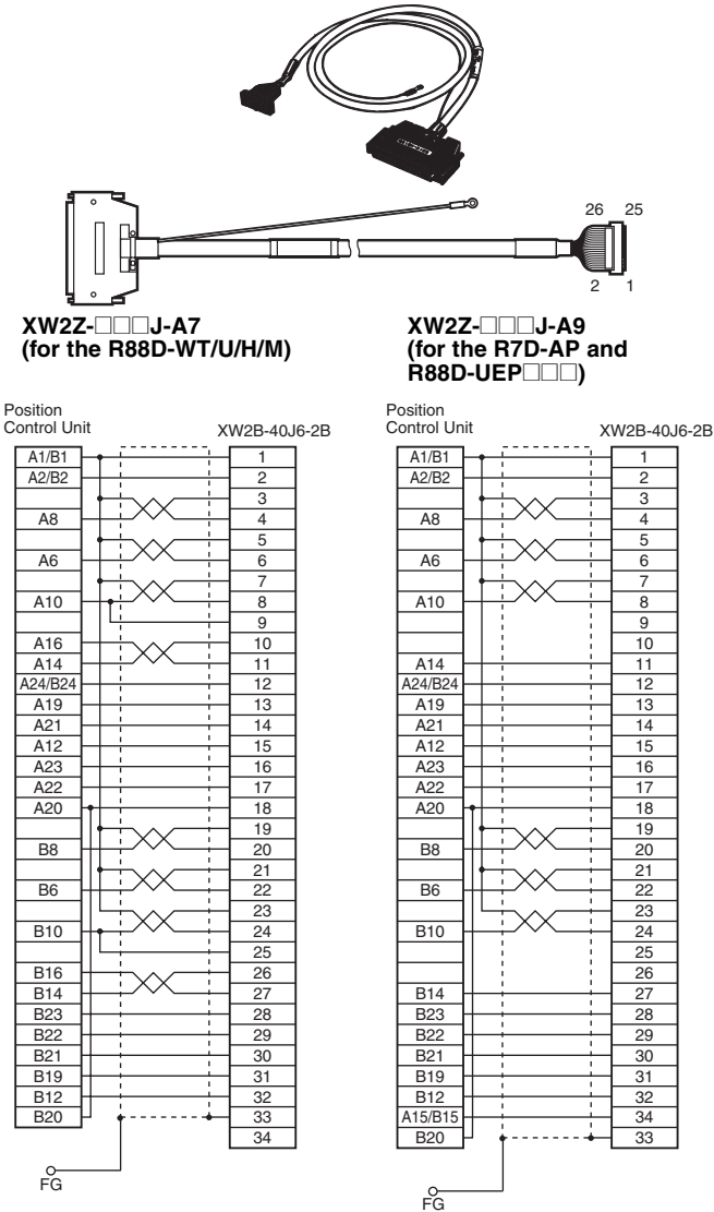
Position Control Unit Connecting Cable
