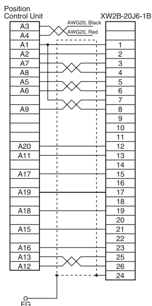
XW2Z-100J-A20 (for the R7D-AP and R88D-UEP□□□)
