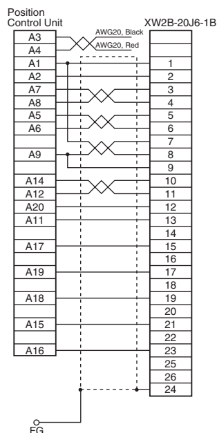
XW2Z-050J-A18 (for the R88D-WT/U/H/M)
