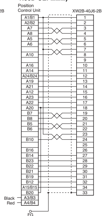
XW2Z-40J6-2B (for the R7D-AP and R88D-UEP0000)
