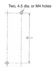
Mounting Holes
