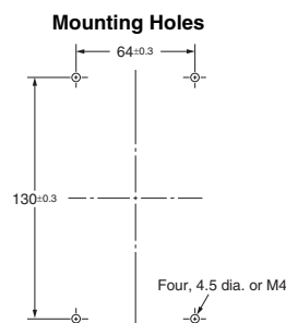
Mounting Holes
