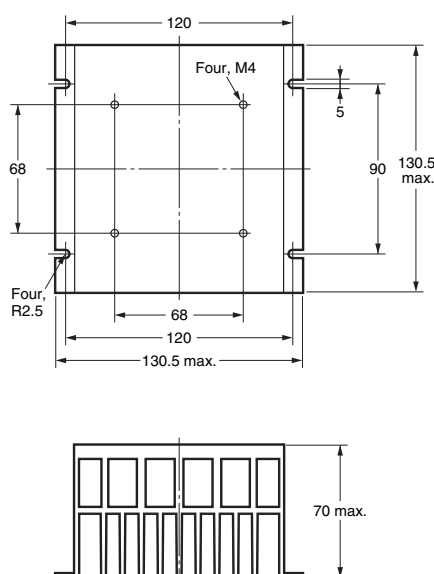
Mounting Holes
