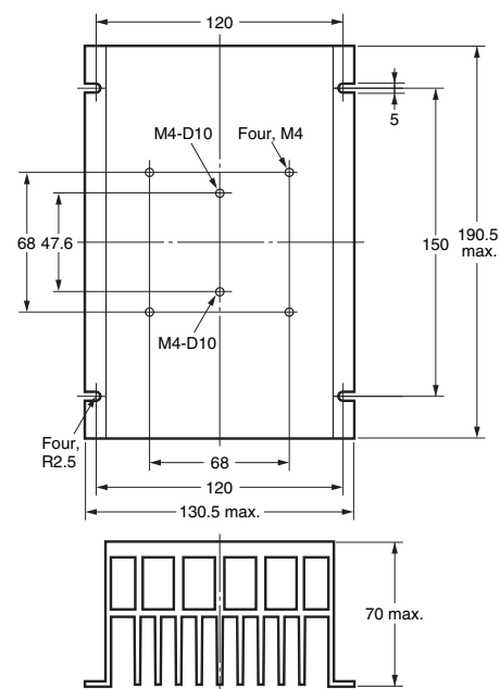
Mounting Holes
