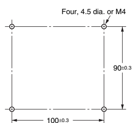
Mounting Holes
