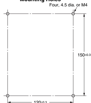
Mounting Holes
