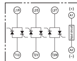
Terminal Arrangement/Internal Circuit Diagram
