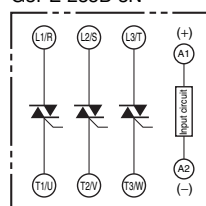
Terminal Arrangement/Internal Circuit Diagram
