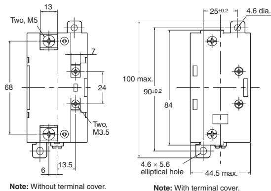
Mounting Holes
