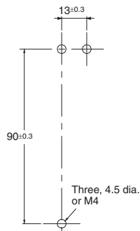
Mounting Holes
