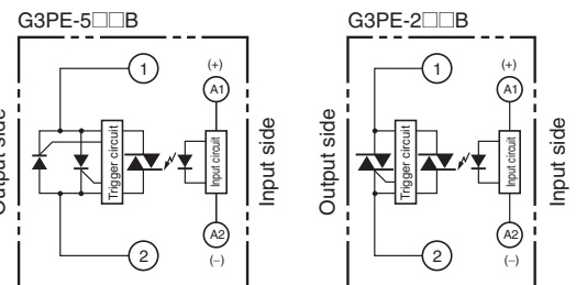
Terminal Arrangement/Internal Circuit Diagram
