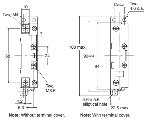
Mounting Holes
