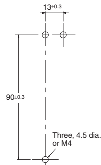
Mounting Holes
