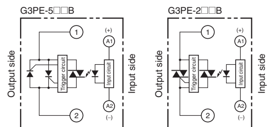
Terminal Arrangement/Internal Circuit Diagram
