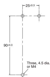
Mounting Holes
