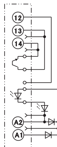
24 V DC Terminal Arrangement/ Internal Connections (Top View)
