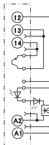
Other Input Voltage Terminal Arrangement/ Internal Connections (Top View)
