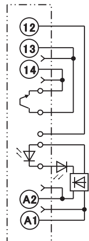
Other Input Voltage Terminal Arrangement/ Internal Connections (Top View)
