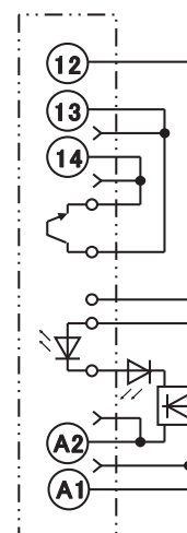
Other Input Voltage Terminal Arrangement/ Internal Connections (Top View)
