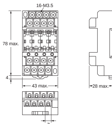
P6BF-4BND (with operation indicator)
