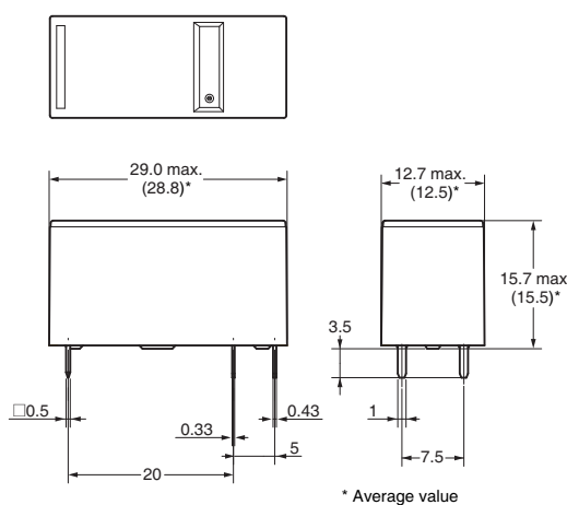
G5RL-1A-E-LN G5RL-1A-E-HR G5RL-1A-E-TV8
