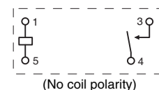
Terminal Arrangement/ Internal Connections (BOTTOM VIEW)
