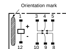
Terminal arrangement/ Internal connections (Bottom view)
