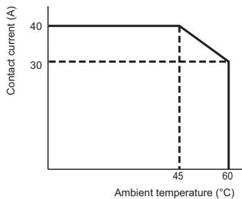
(Fig. 1) Ambient temperature and rated carry current of the main contact
