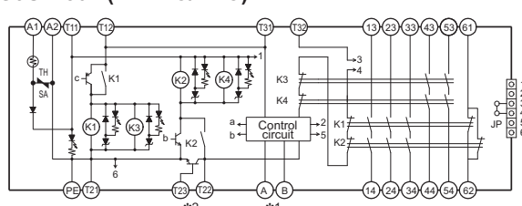
G9SA-321-T□ (24 VAC/VDC)
