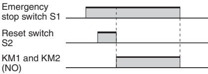
Timing Chart
