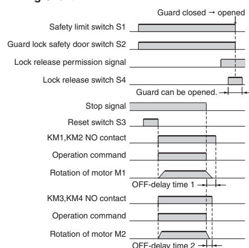
Timing Chart
