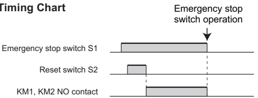
Timing Chart
