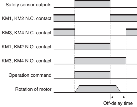
Timing chart
