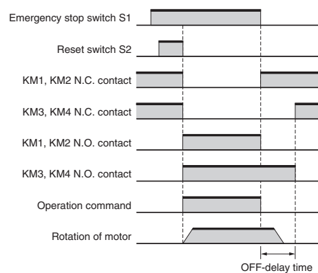
Timing chart
