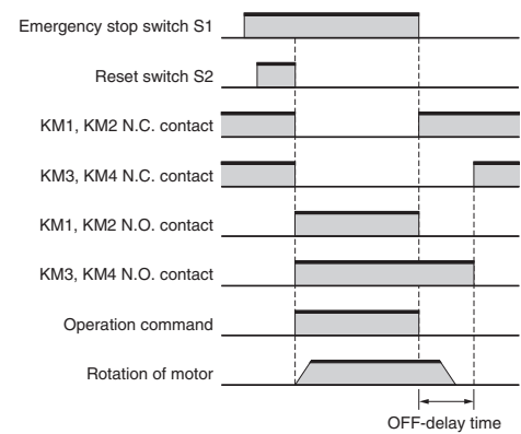
Timing chart
