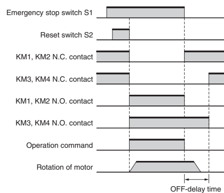
Timing chart
