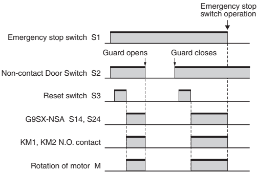
Timing chart
