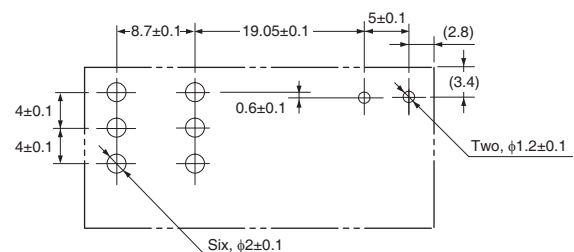
Terminal arrangement/Internal Connection (BOTTOM VIEW)
