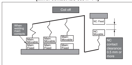
[Mirror contact IEC 60947-4-1]
