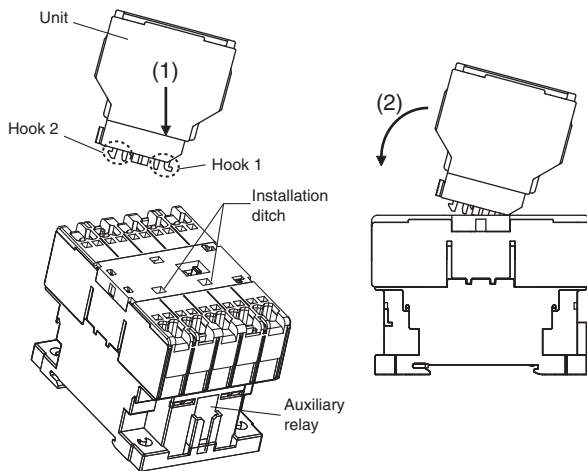
Diagram 1. Mounting method
