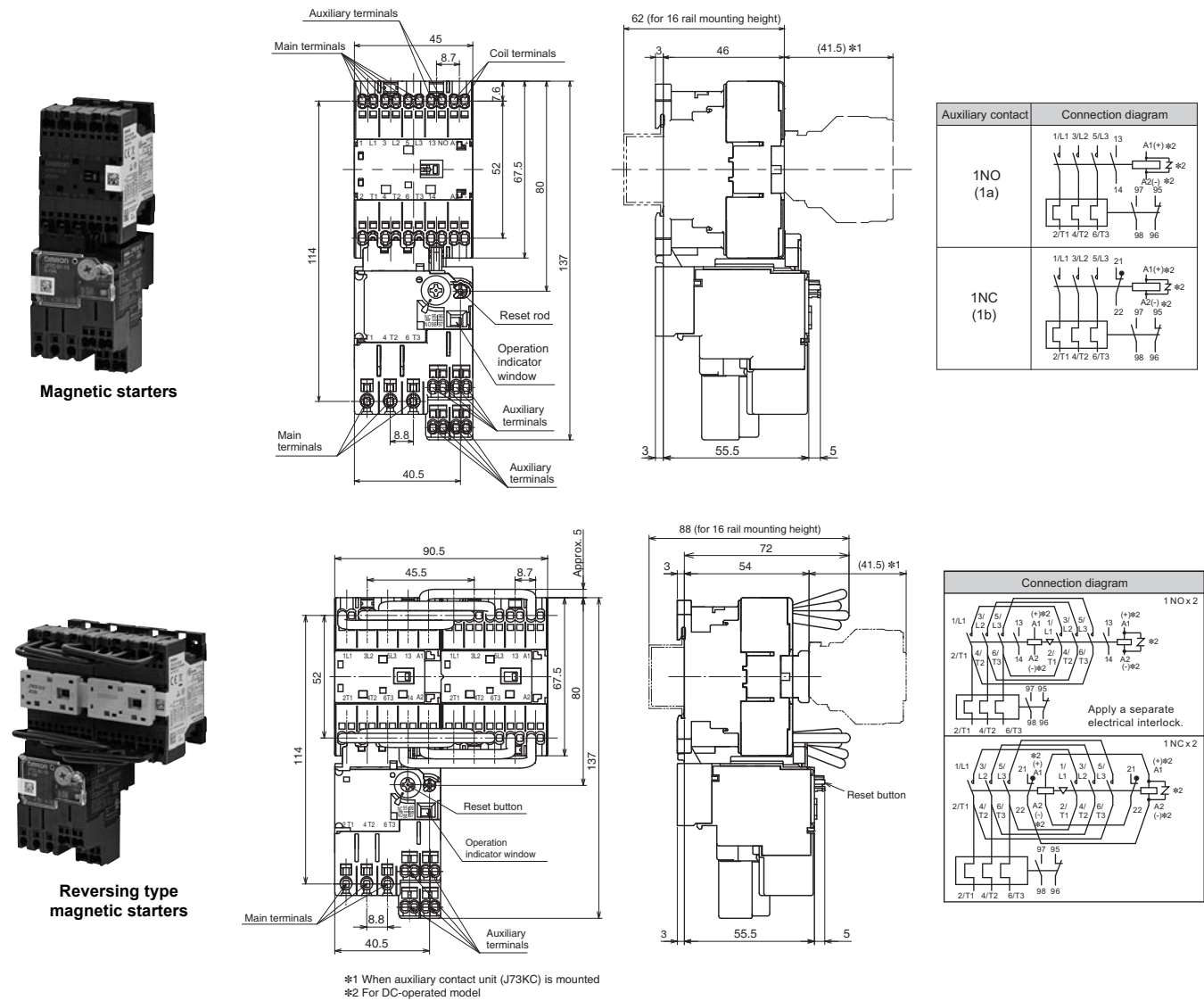
Product main unit arrangement
