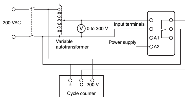
Connection Diagram
