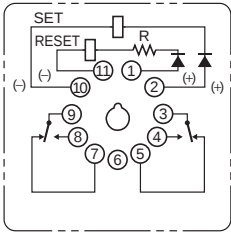
Terminal Arrangement/Internal Connections (Bottom View)
