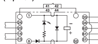
Terminal Arrangement/Internal Connection Diagram (Top View)
