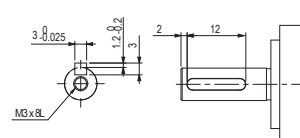
Shaft end
