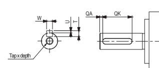
Shaft end
