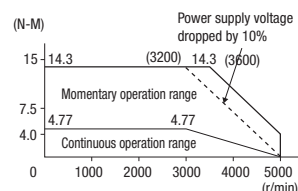
R88M-K1K530H/T (1.5 kW)
