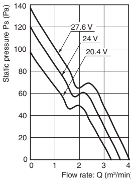
R89F-DS1225H
