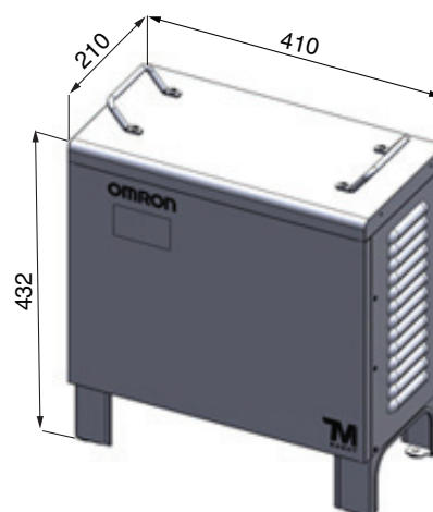
Control Box
