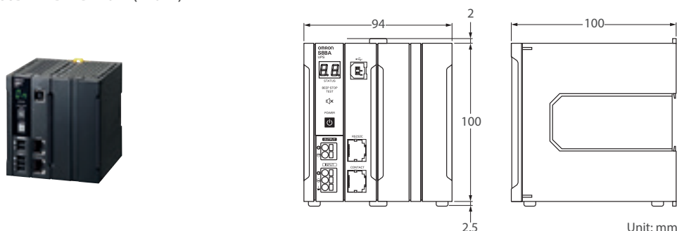
S8BA-24D24D240LF (240 W)
