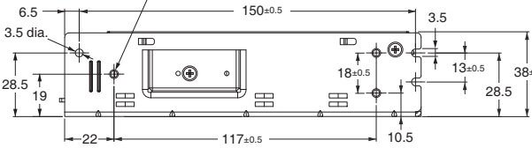
Panel mounting holes dimensions
