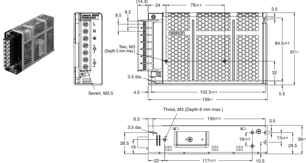
Panel mounting holes dimensions
