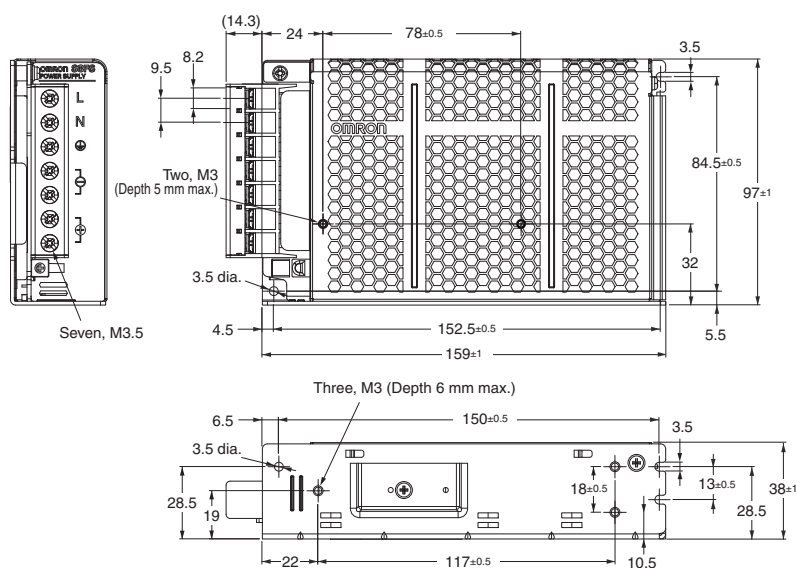
Panel mounting holes dimensions
